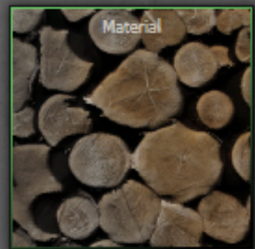
Wood_Ends 51 instructions
