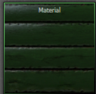
Wood_Boards_Green 47 instructions
