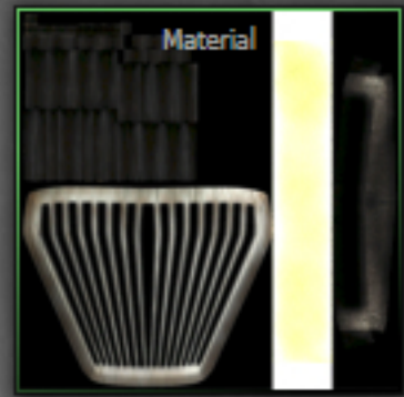
atv_headlight 32 instructions
