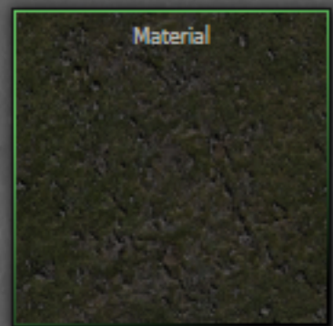
Rocky_Grass 49 instructions
