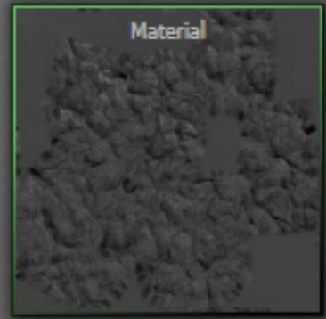
Boulder_01 51 instructions
