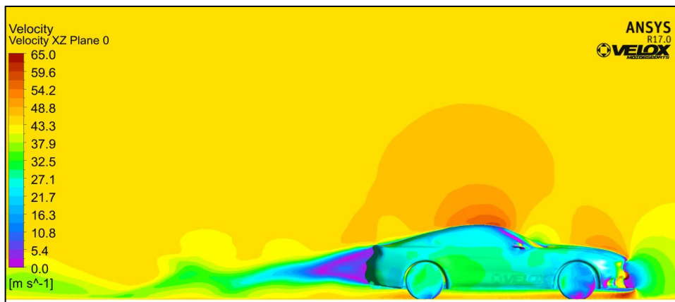
Figure 1.3.4: Ventus1 Mustang – Velocity Cut Plane
