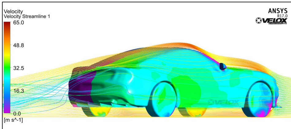
Figure 5.7.5: Streamlines Off the Diffuser
