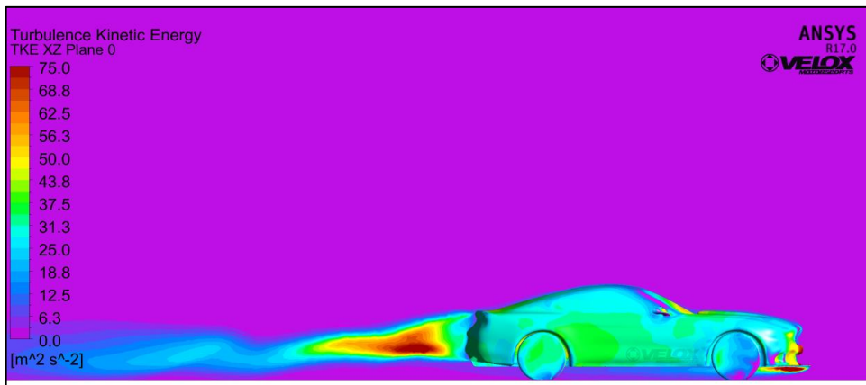
Figure 5.5.1: TKE Plot Symmetry Plane
