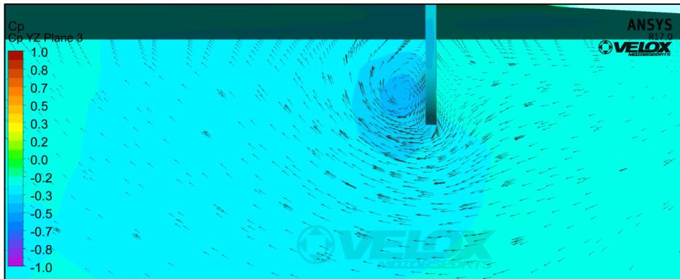
Figure 5.7.3: Vortex Formation on Strake
