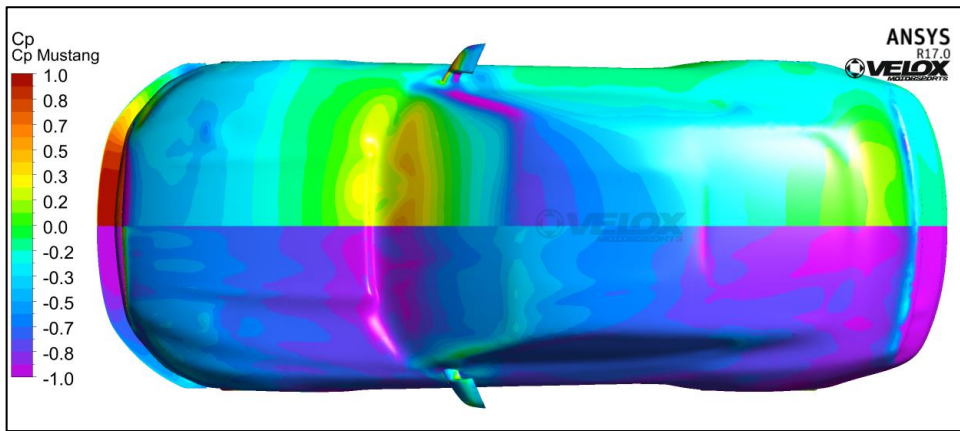
Figure 5.3.3: Cp & Wall Shear Top
