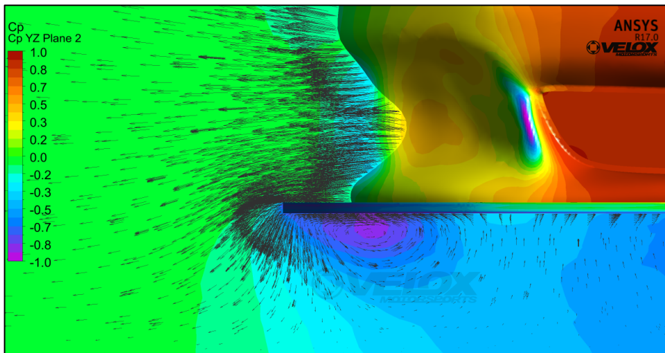
Figure 1.3.4: Vortex Formation under Splitter
