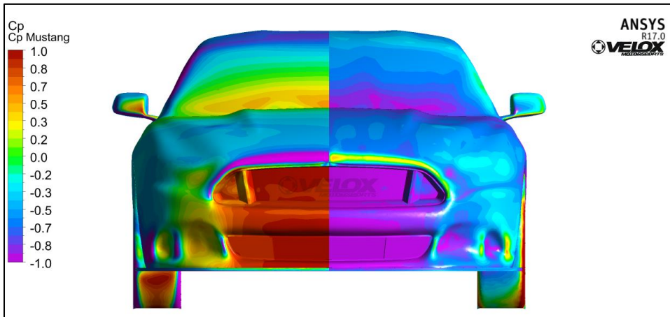
Figure 5.3.1: Cp & Wall Shear Front
