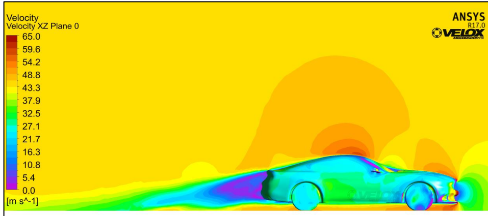
Figure 1.3.3: Stock Mustang – Velocity Cut Plane
