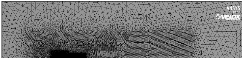
Figure 2.4.2: Mesh Wake Zone Refinement
