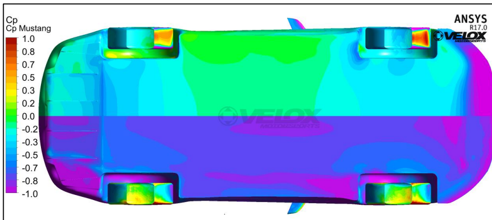
Figure 5.3.4: Cp & Wall Shear Bottom
