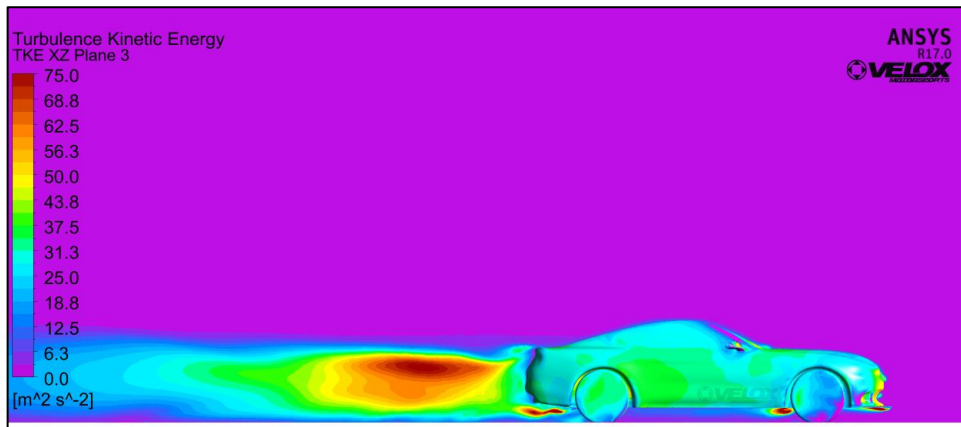
Figure 5.5.4: TKE Plot XZ Plane 3 (Offset from Sym Plane 0.5m)
