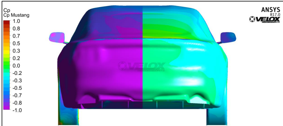
Figure 5.3.2: Cp & Wall Shear Rear
