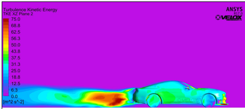
Figure 5.5.3: TKE Plot XZ Plane 2 (Offset from Sym Plane 0.3m)
