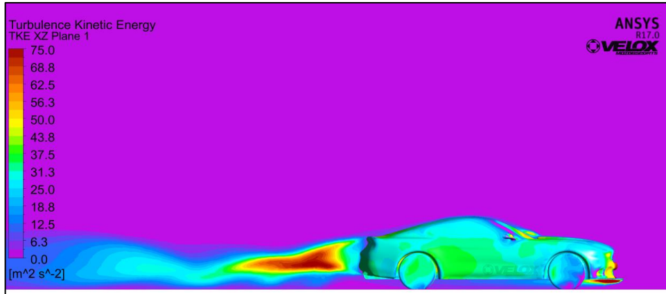
Figure 5.5.2: TKE Plot XZ Plane 1 (Offset from Sym Plane 0.1m)
