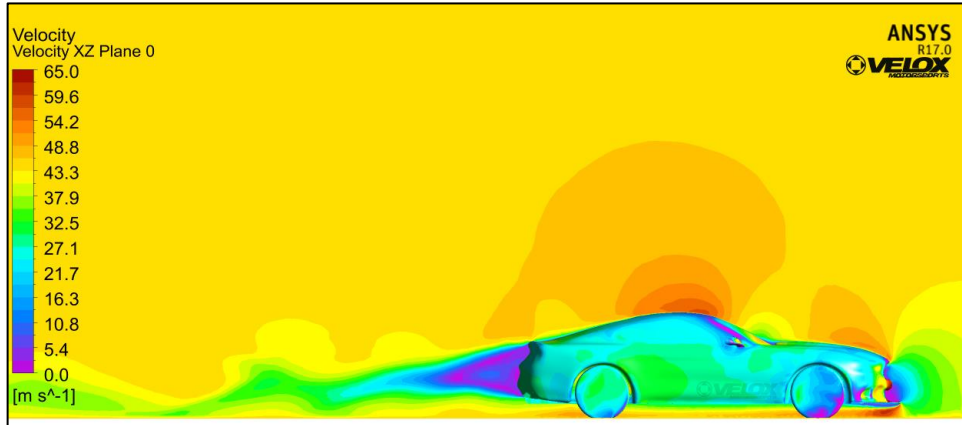
Figure 5.4.1: Velocity Plot Symmetry Plane
