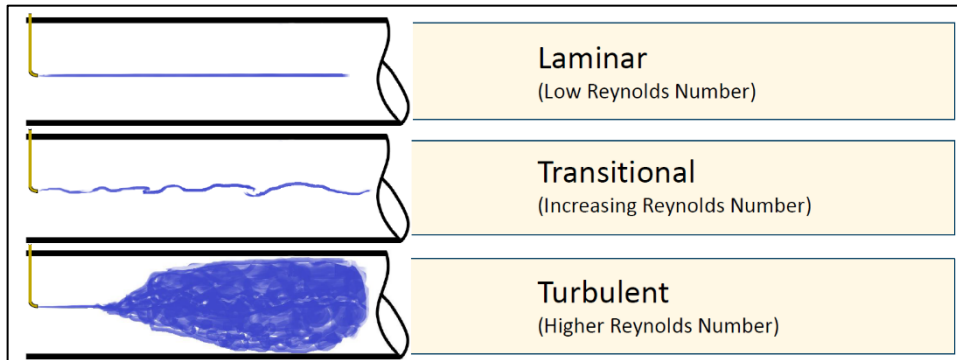
Figure 3.3.1: Flow Classifications
