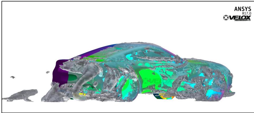
Figure 5.7.1: Q-Criterion Displays Vortices off the Mustang
