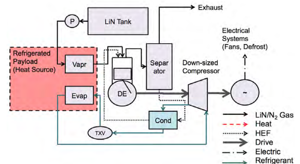
Figure 5: Dearman transport refrigeration system
