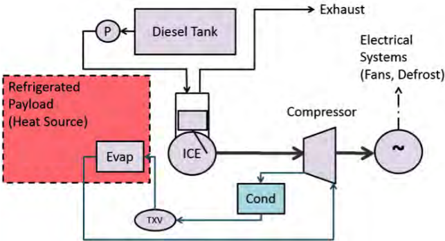
Figure 7: Auxiliary diesel engine powered TRU diagram
