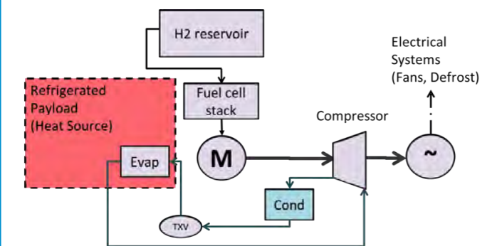
Figure 11: Hydrogen fuel cell TRU
