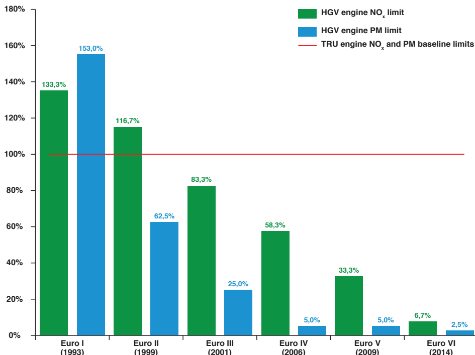
Figure 1: Euro truck engine emission standards compared to the proposed NRMM Stage 5 TRU standard. Source: European Commission; DieselNet. 9
