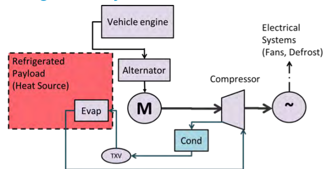
Figure 8: Alternator driven from vehicle engine powered TRU diagram
