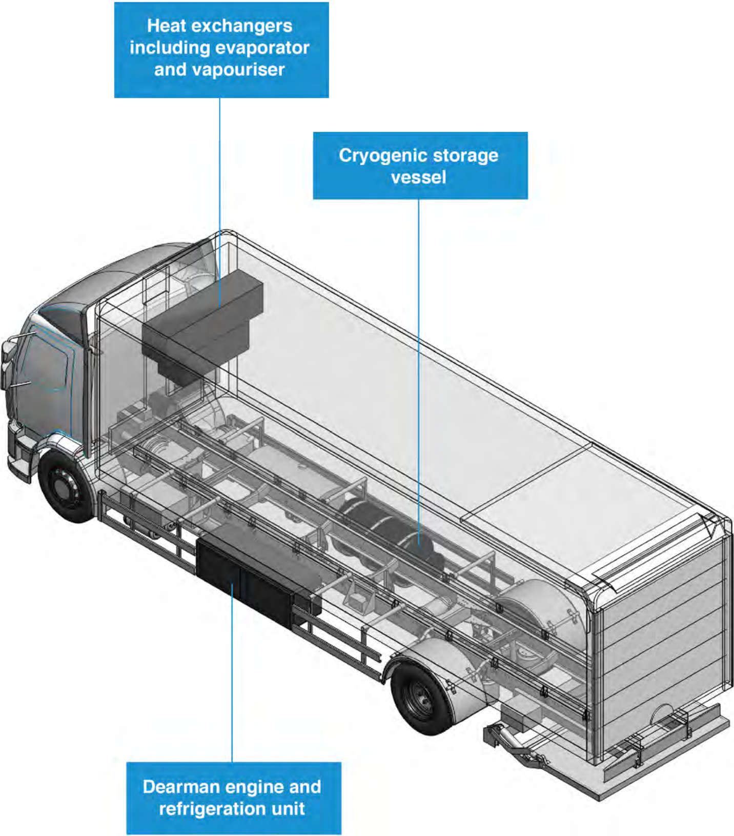
Figure 6: The Dearman transport refrigeration system
