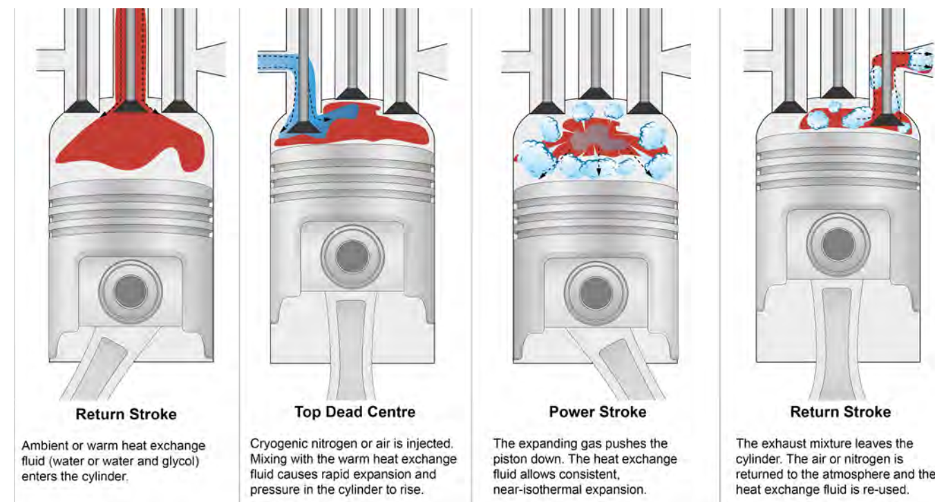
Figure 3: The Dearman engine power cycle.
