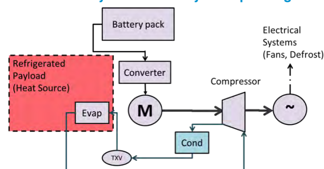
Figure 10: All-electric TRU
