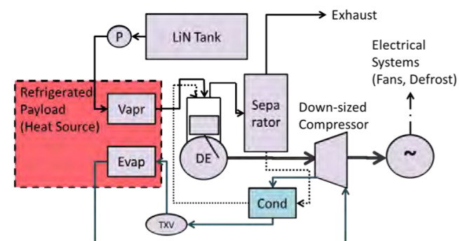
Figure 9: Dearman engine powered TRU
