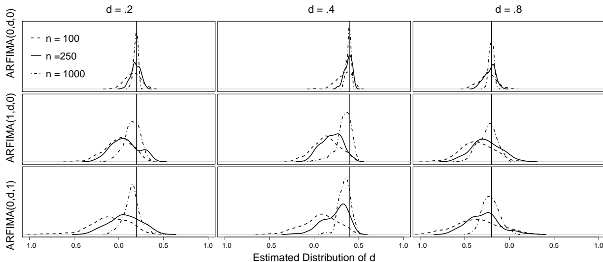
Figure 1: Distributions of Estimates for d
