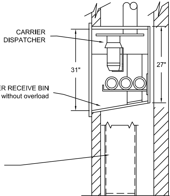
SIDE SECTION
