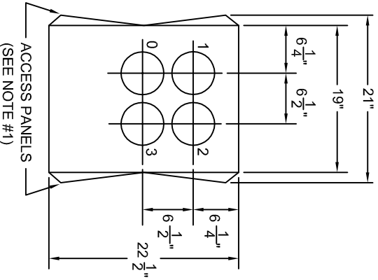
4-PORT SIDE
